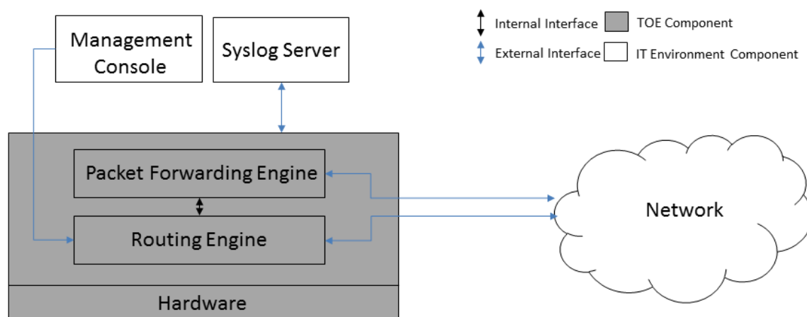
Figure 1 TOE Boundary
